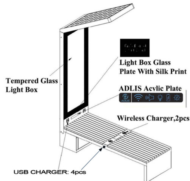
Solar Panel,22V,135W
