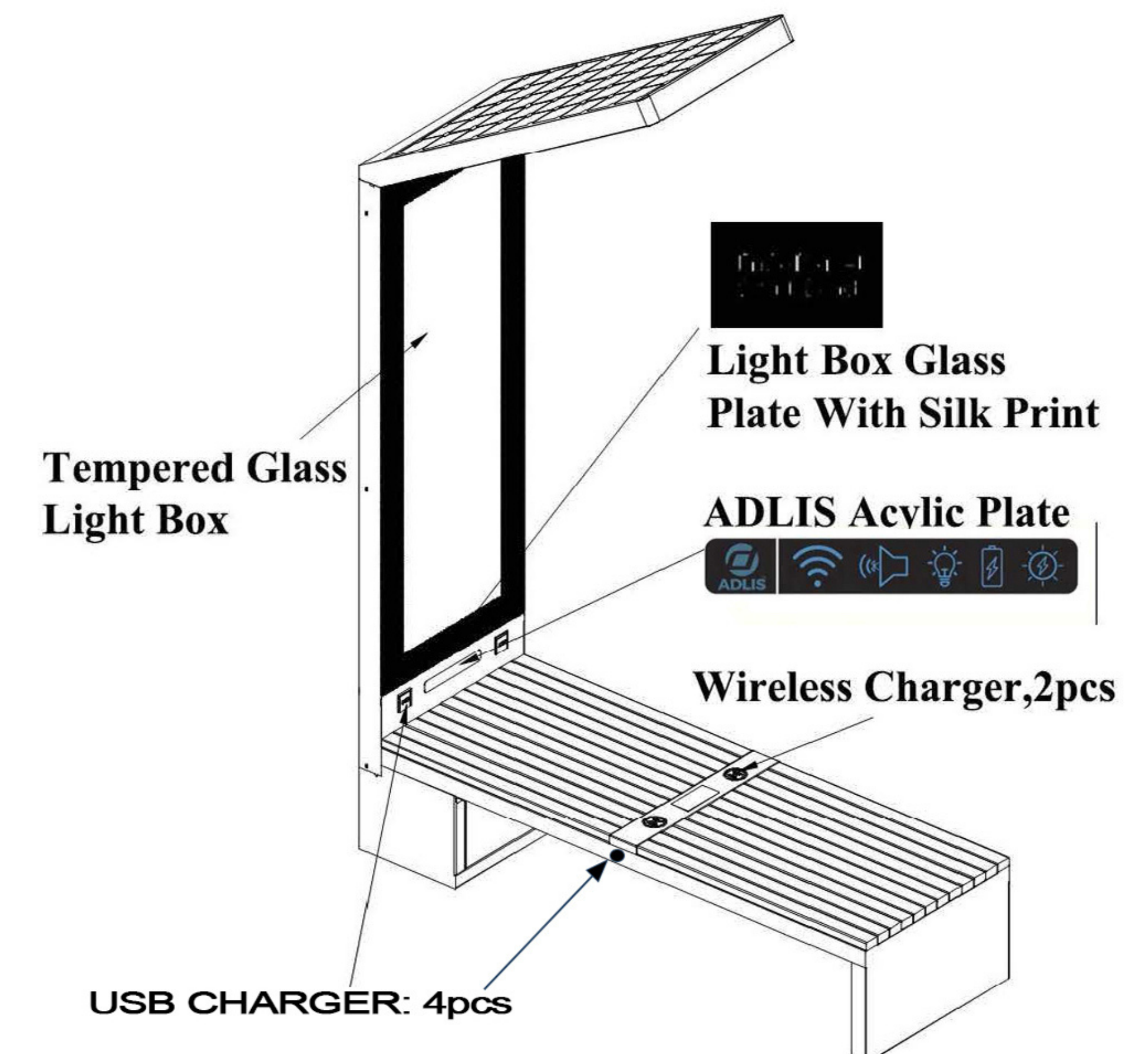
Solar Panel,22V,135W
